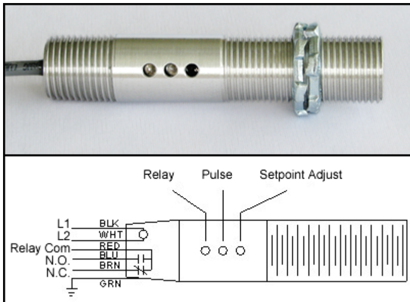
Figure 2. LED Indicators and Wire Color Code
