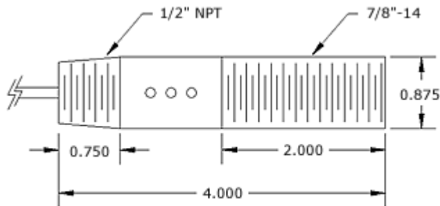
Figure 5. Dimensions (in inches)
